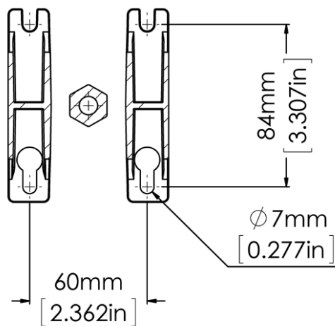
SECTION Z-Z
